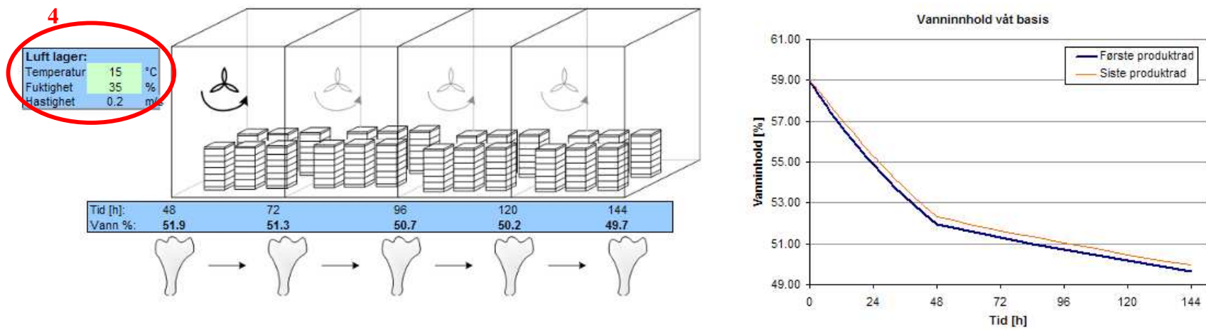
Figur 2-1: GUI
