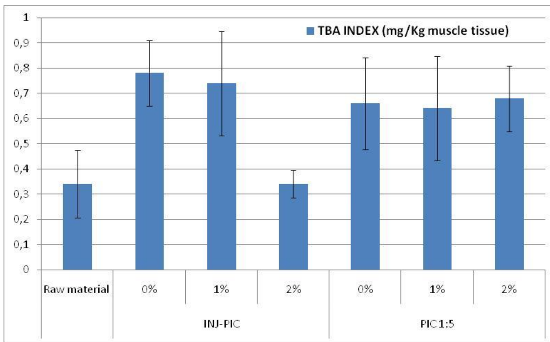
Figure 3.48. TBARS levels in heavy salted fish. For the two salting methods 0, 1 or 2 % phosphate were tested. Means and standard deviations of five fish are shown.
