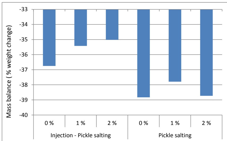
Figure 3.45. Mass balances for water content in heavy salted split fish. For the two salting methods 0, 1 or 2 % phosphate were tested. Means of three fish are shown.
