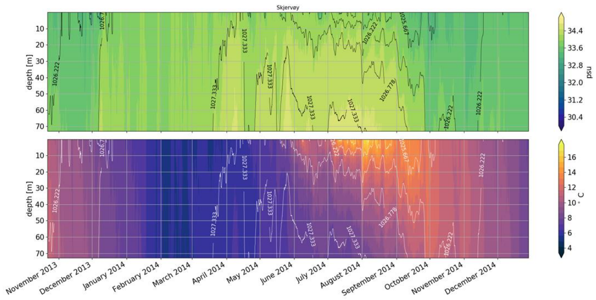
Figure 20. Salinity (upper), temperature (lower) and density (contours) at the release point at Indre Skjervøy. Stratification is strong where the density contours are close together.
