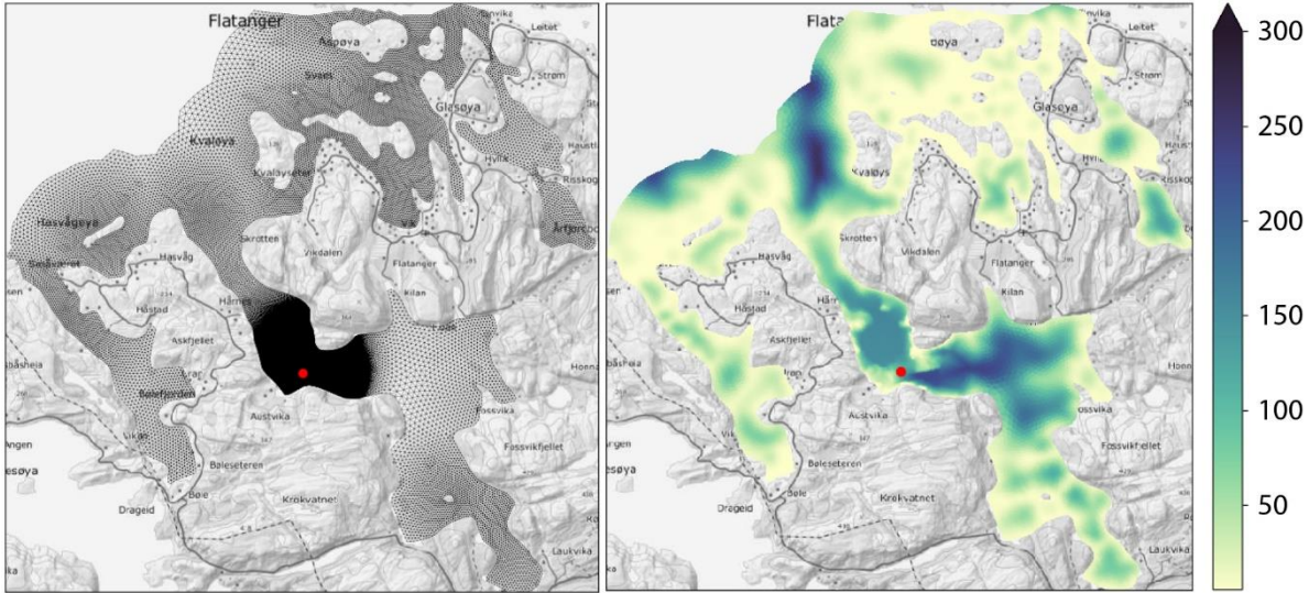
Figure 16. The mesh (left) and bottom topography (right) for Austvika. The red point shows the location of the release of H_2O_2 .
