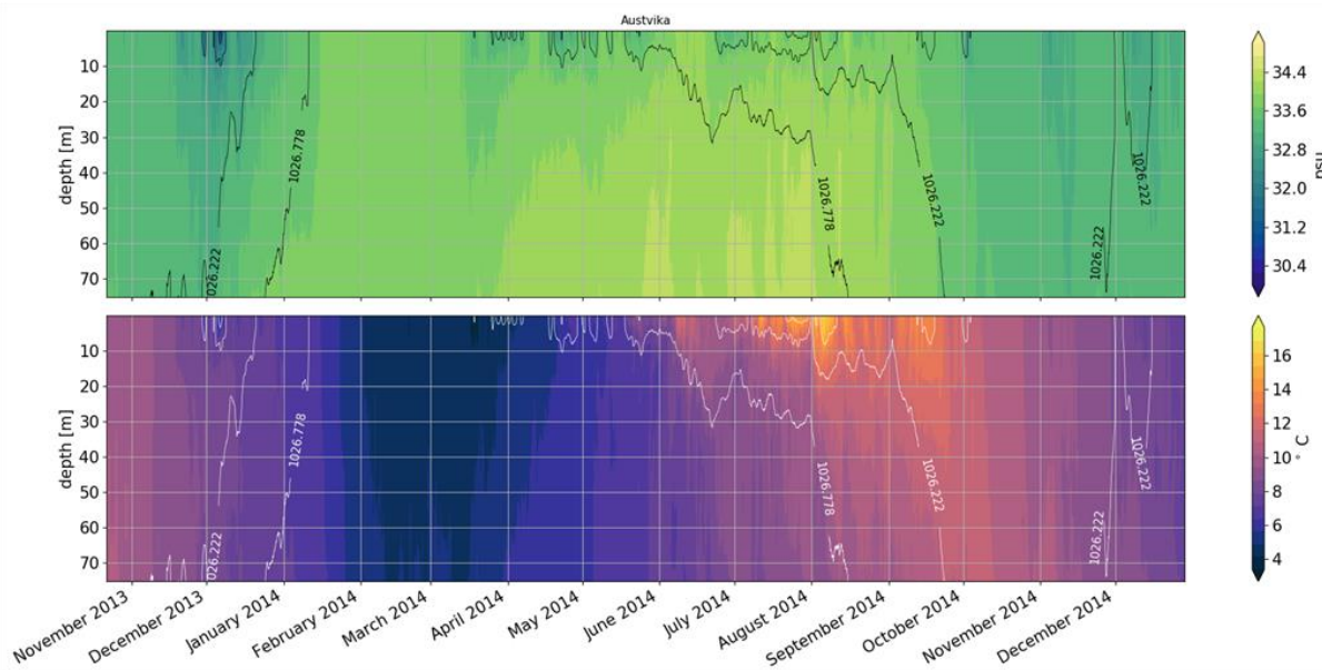
Figure 21. Salinity (upper), temperature (lower) and density (contours) at the release point at Austvika. Stratification is strong where the density contours are close together.
