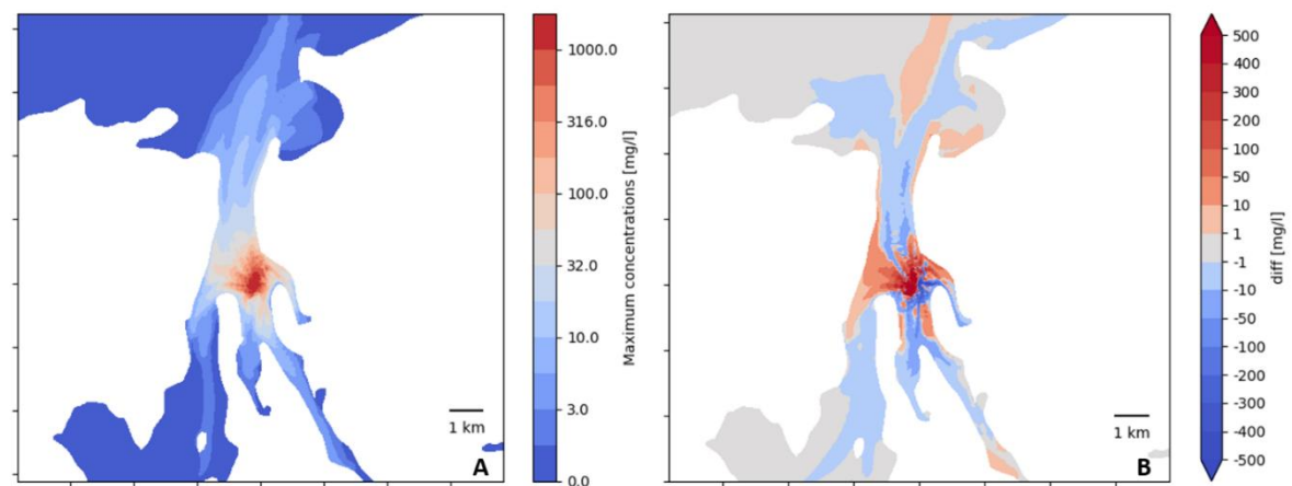
Figure 57. Same as Figure 55 for Kjerneset.
