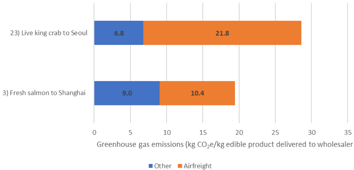
Figure 4-3 Greenhouse gas emissions of air freighted products.
