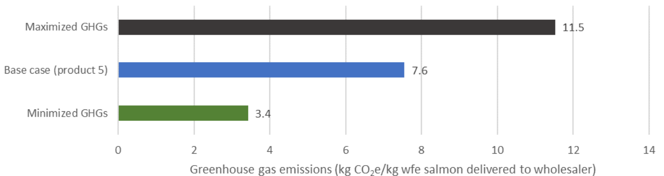
Figure 5-3 Change in greenhouse gas emissions of fresh salmon fillet to Paris when a number of parameters are varied, including the feed conversion ratio, the sourcing of soy, by-product utilization, energy intensity in various steps and the load on return trips.
