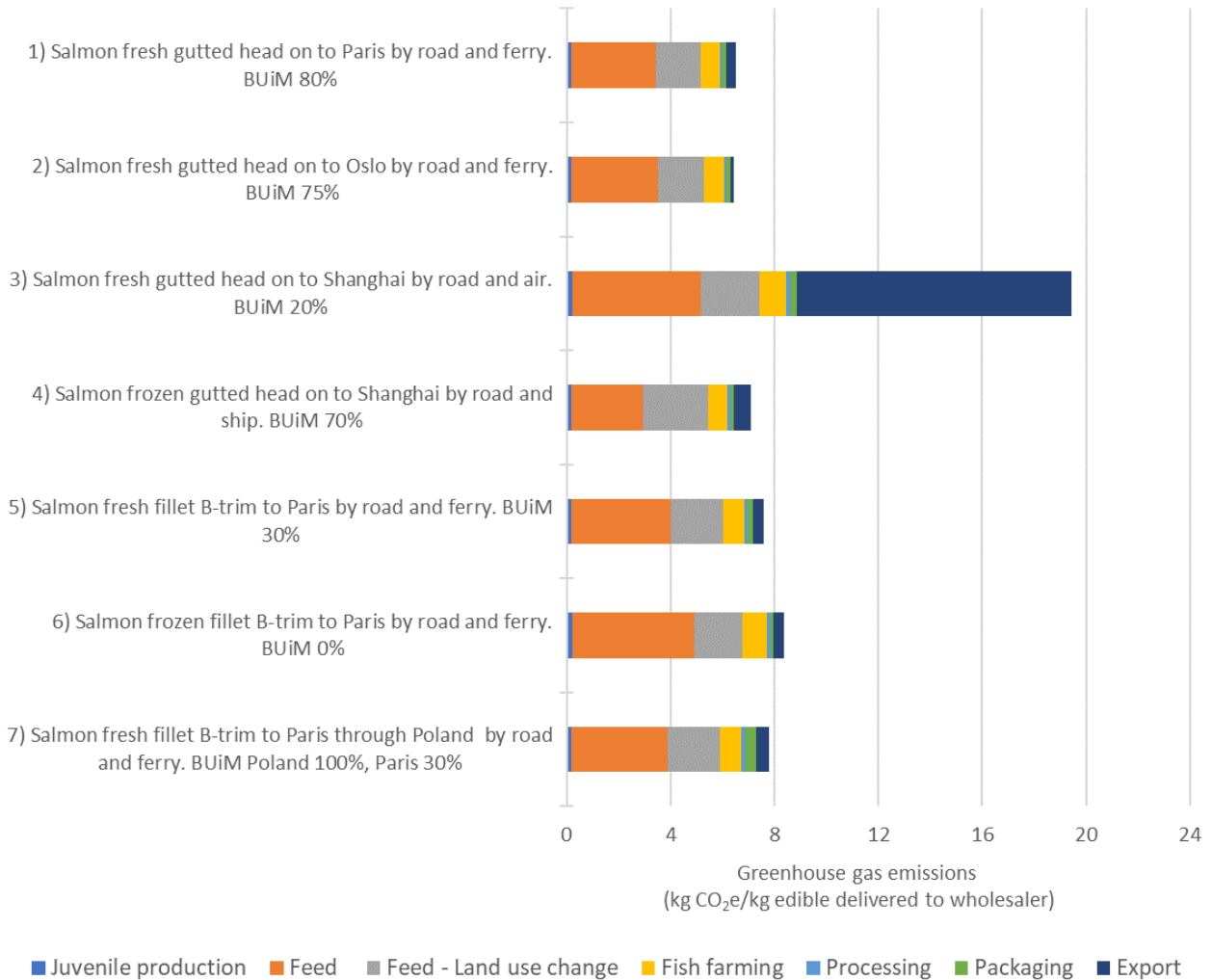
Figure 4-4 Greenhouse gas emissions of all salmon products (kgCO 2 e/kg edible product at wholesaler) BUiM = By-product use in market.
