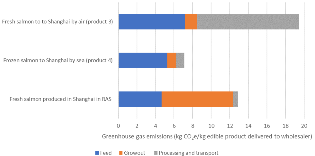
Figure 5-7 Comparison of fresh and frozen salmon products shipped and flown to China from Norway or produced in a recirculating aquaculture system in China.
