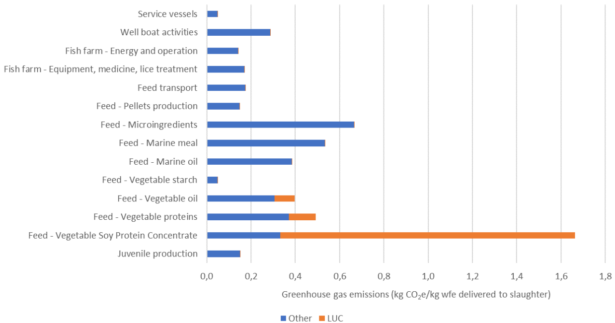
Figure 4-5 Detailed greenhouse gas emissions per kilo farmgate salmon of different activities and feed inputs, indicating the contribution from direct Land Use Change separately.
