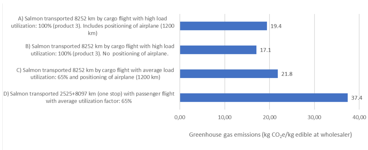
Figure 5-10 Greenhouse gas emission of alternative airfreight scenarios.
