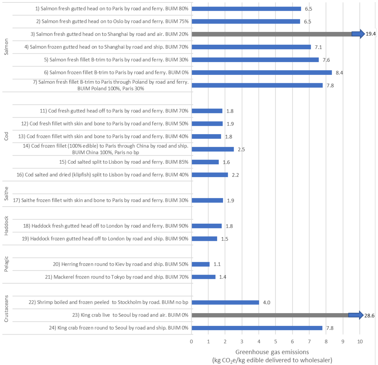
Figure 1 Greenhouse gas emissions of all studied products (kg CO 2 e/kg edible product delivered to wholesaler) BUiM = By-product use in market.
