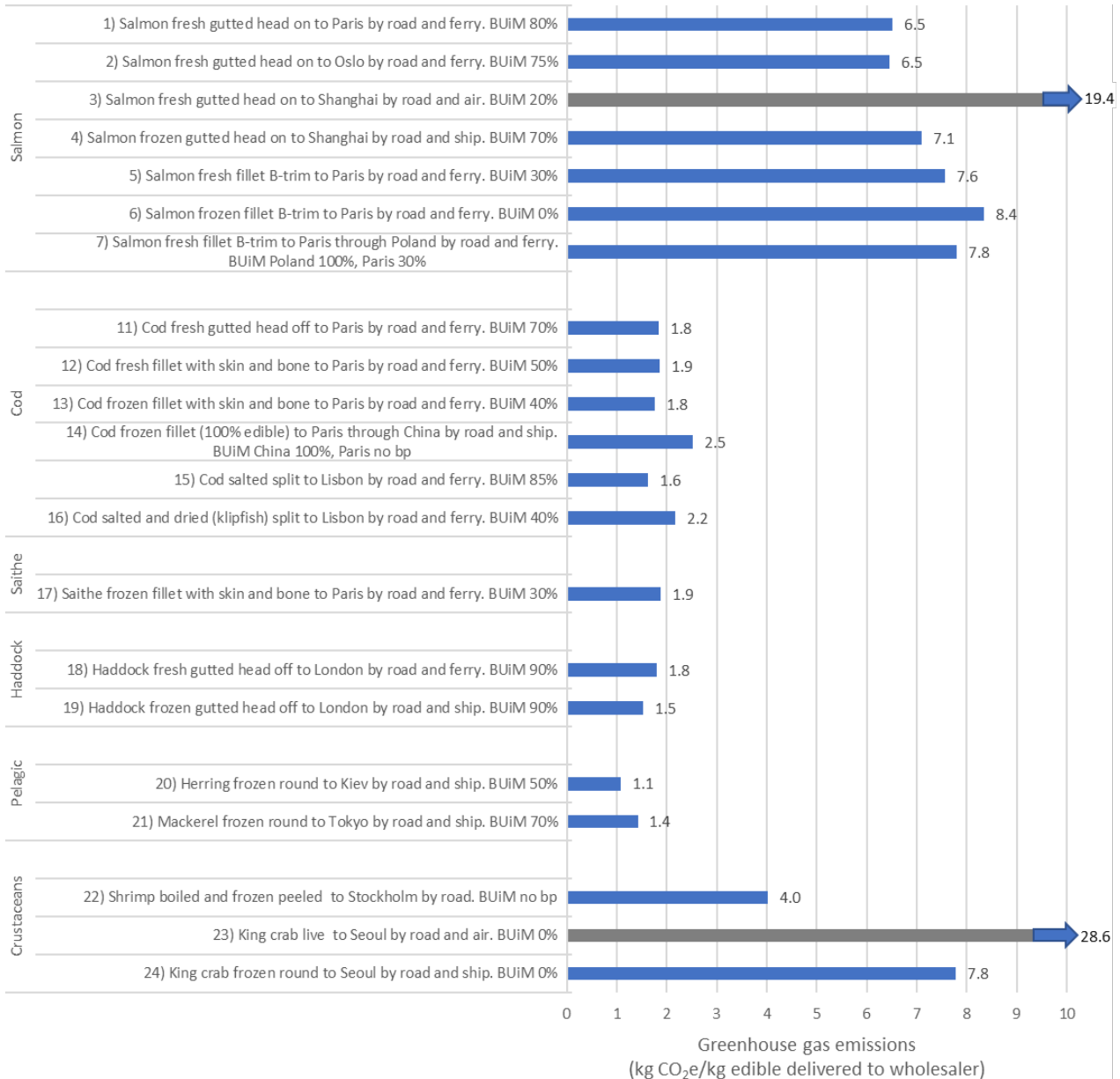
Figure 4-2 Greenhouse gas emissions of all studied products (kg CO 2 e/kg edible product delivered to wholesaler) BUiM = By-product use in market.
