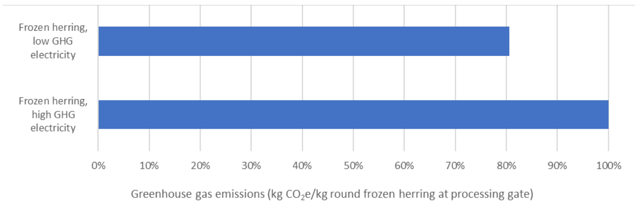
Figure 5-9 Change in CF of round frozen herring at the processing gate when electricity is modelled as Norwegian electricity with certificate of origin rather than average European electricity.
