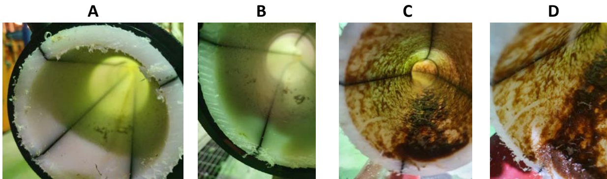
Figure 11: Photographs taken after dissecting the pipe bend for the erosion study: a view into the straight line before the bend (A), into the bend inlet (B), into the bed outlet (C) and into the straight section after the bend (D).
