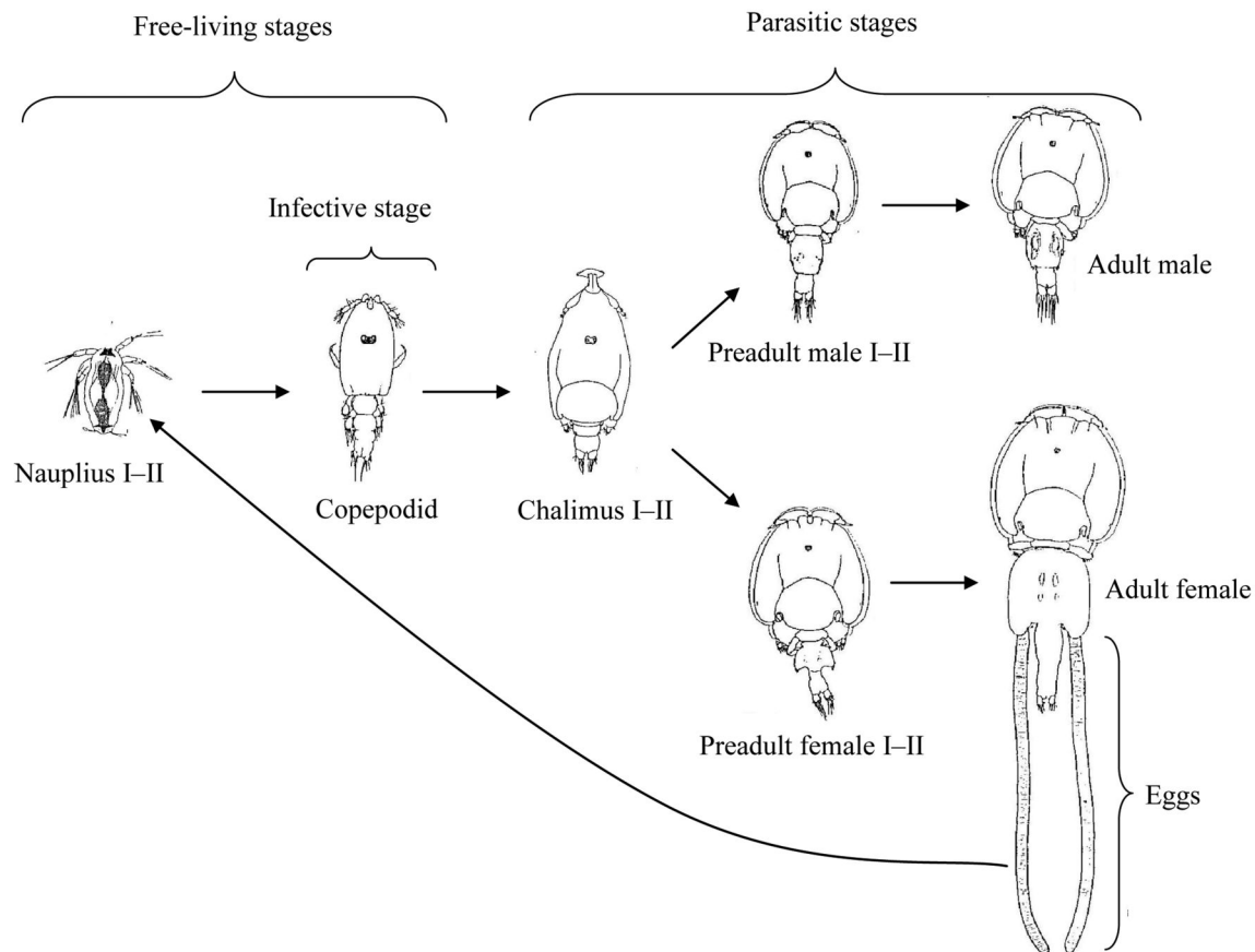
Figure 1. The life cycle of L. salmonis consisting of eight developmental stages, including 3 free-living and 5 parasitic attached to the host (Hamre et al., 2013; modified by Igboeli et al., 2014).
